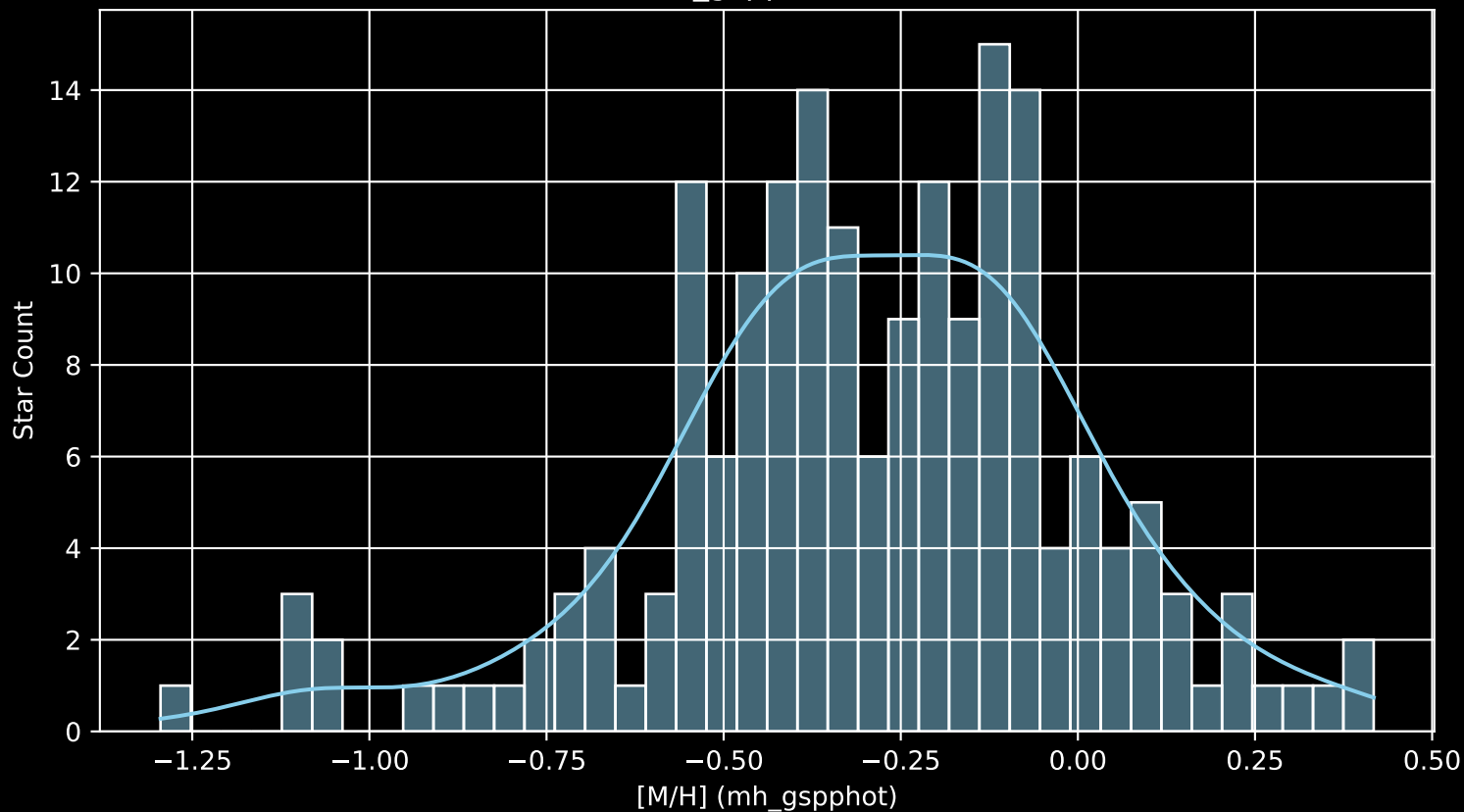
APOGEE DR17 Field: [158+63_MGA [M/H] (mh_gspphot) (n= 184)
