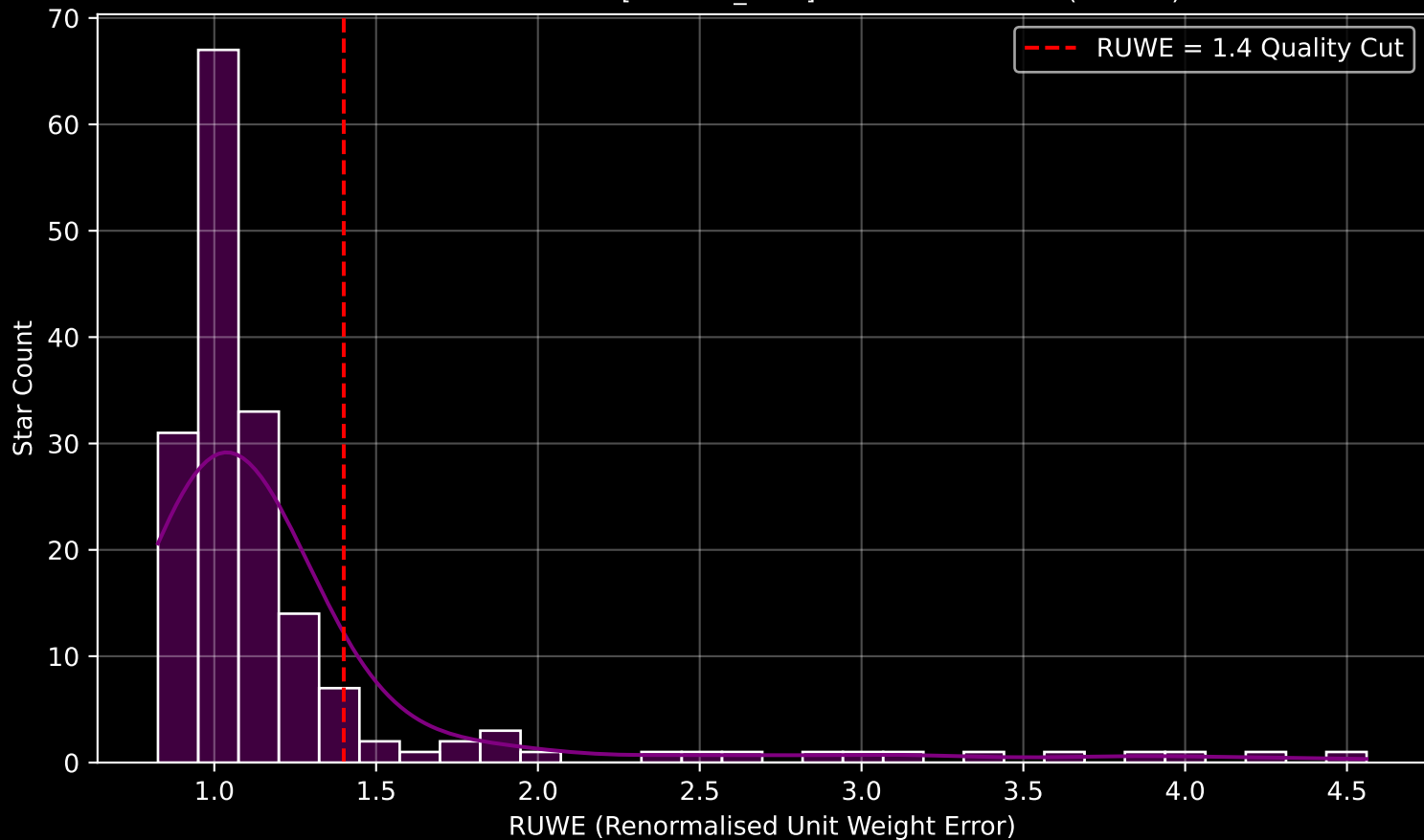
GAPOGEE DR17 Field [158+63_MGA] RUWE Distribution (n= 173)
