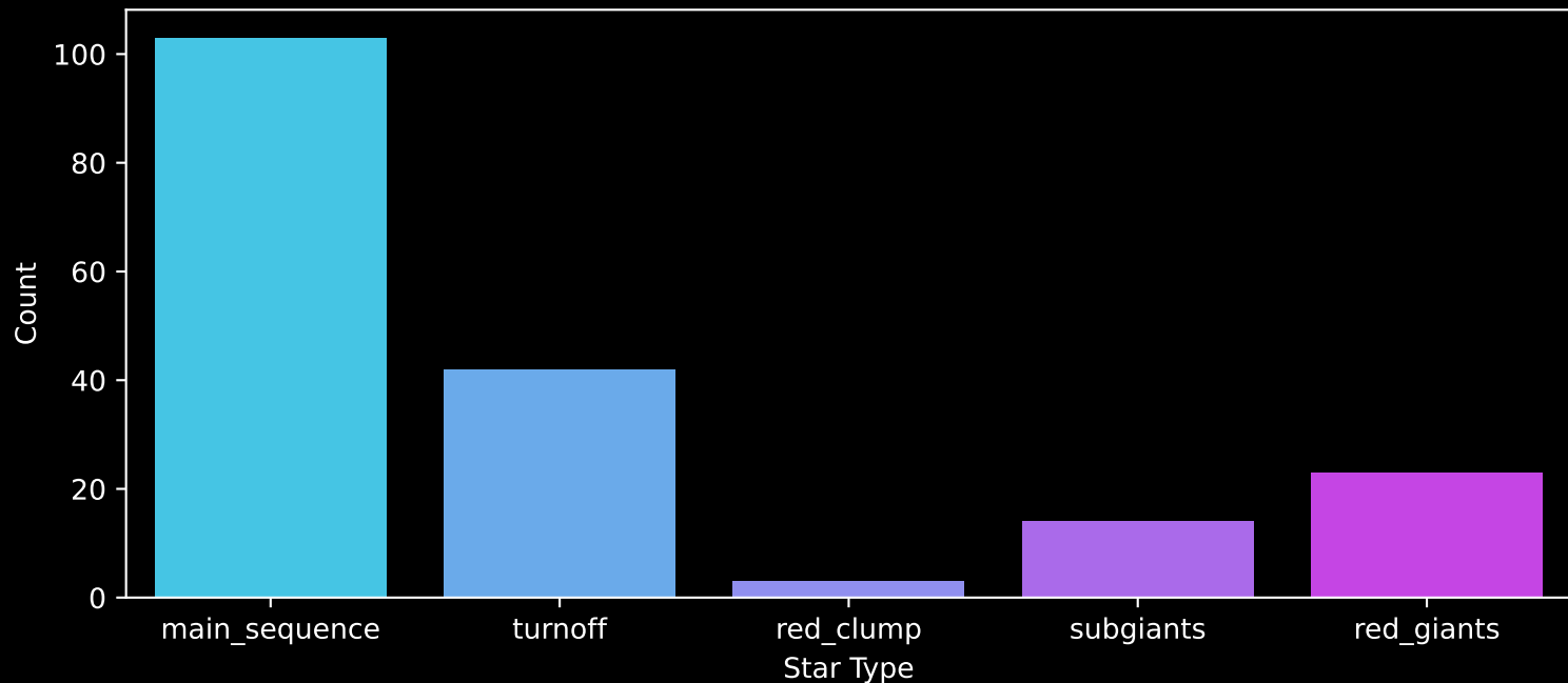
APOGEE DR17 Field: [158+63_MGA] Count plot of Star Type
