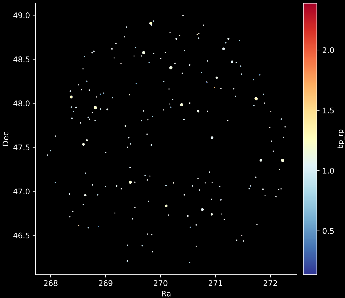
APOGEE DR17 Field: [158+63_MGA] Stars: 185
