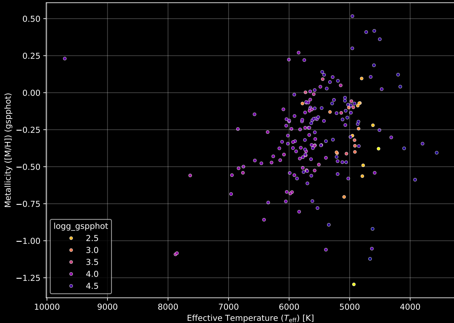
APOGEE DR17 Field: [158+63_MGA] Stellar Population Parameters (n= 185)
