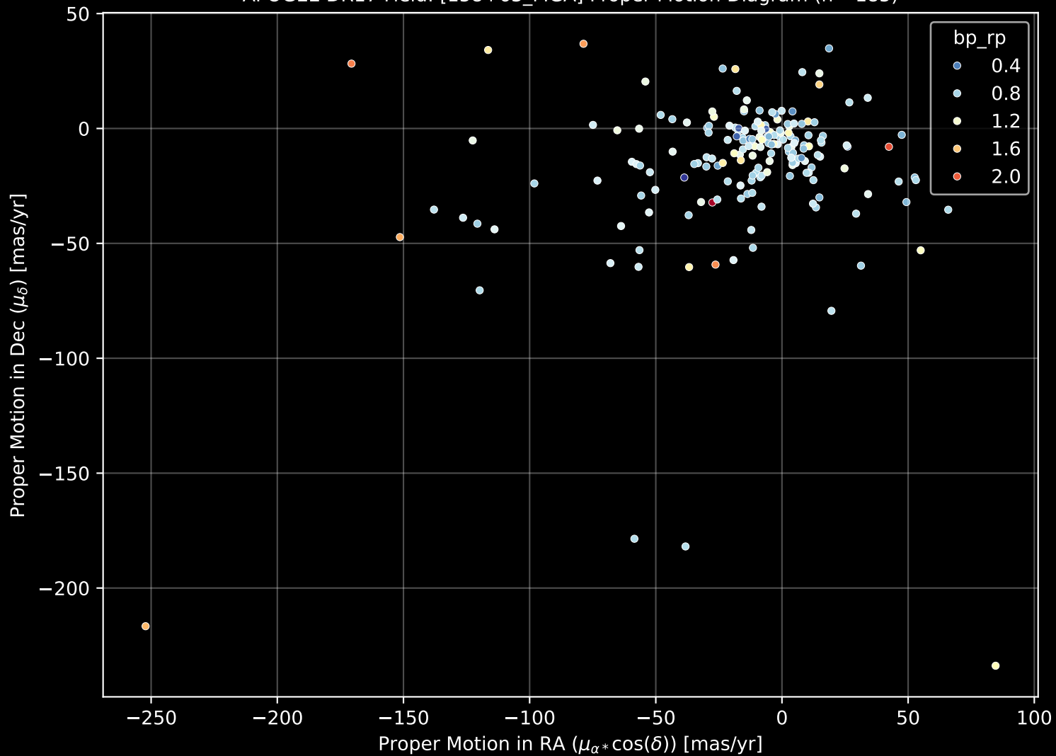
APOGEE DR17 Field: [158+63_MGA] Proper Motion Diagram (n= 185)
