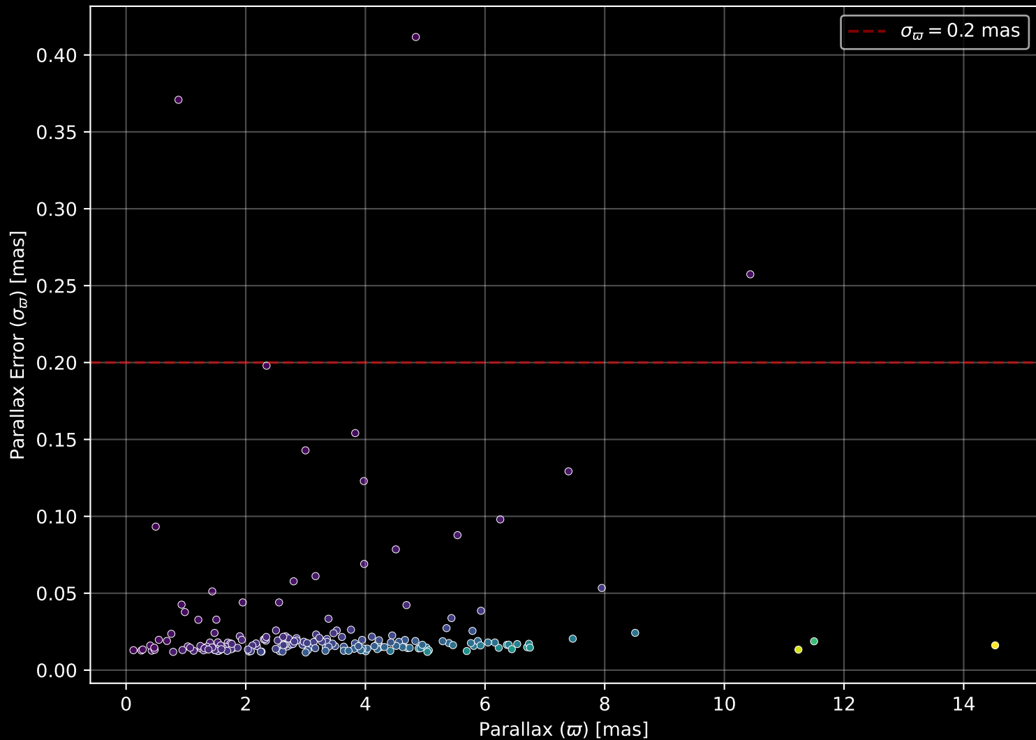
APOGEE DR17 Field: [158+63_MGA] Parallax Quality (n= 185)
